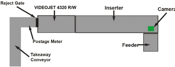
Sample inserter with feeder, vision system, JET MAIL III Read/Write, postage metre, and takeaway conveyor layout
