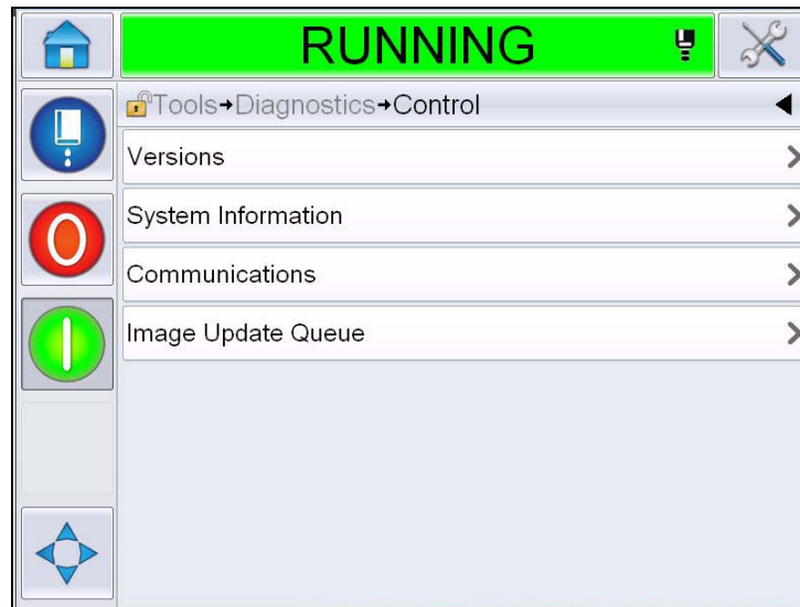
Figure 5-20: Control Parameters
