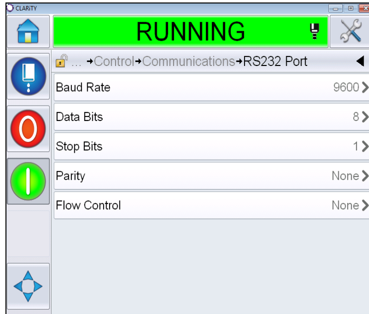
Figure 4-12: Serial Port
