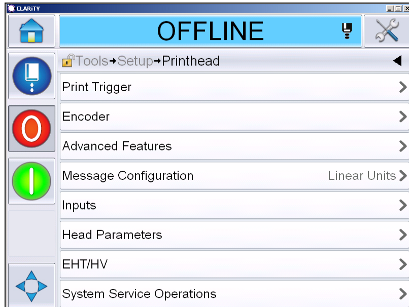
Figure 4-14: Printhead Menu
