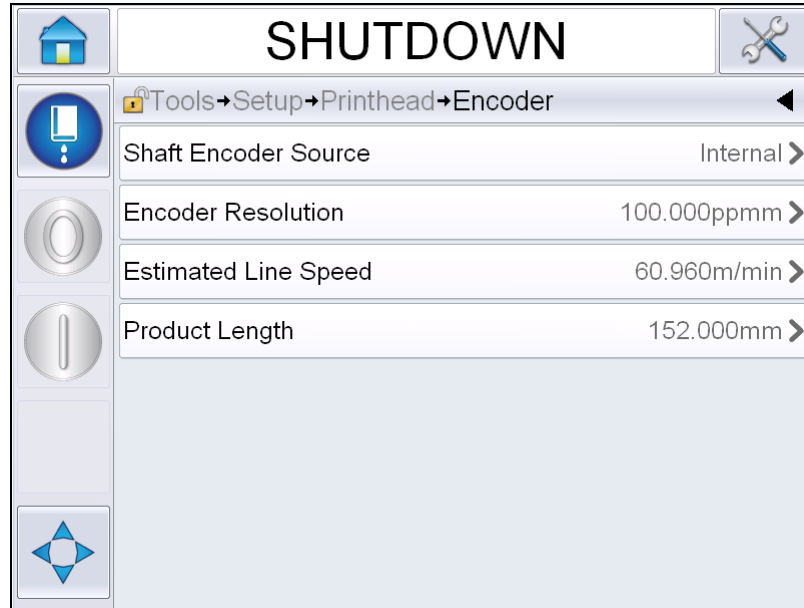
Figure 4-16: Encoder Menu
