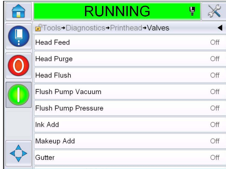
Figure 5-18: Valves
