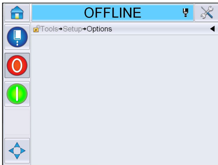
Figure 5-7: Options Page
