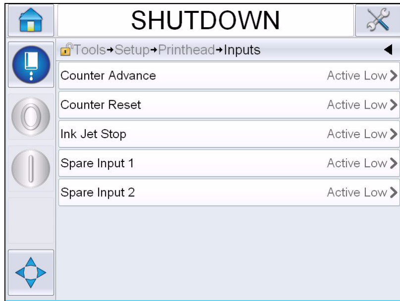
Figure 4-19: Inputs Menu
