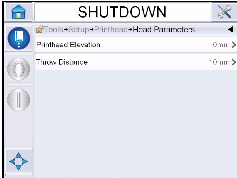
Figure 4-20: Head Parameters Menu
