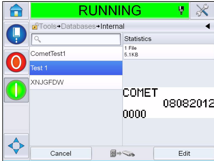
Figure 5-52: Internal Screen
