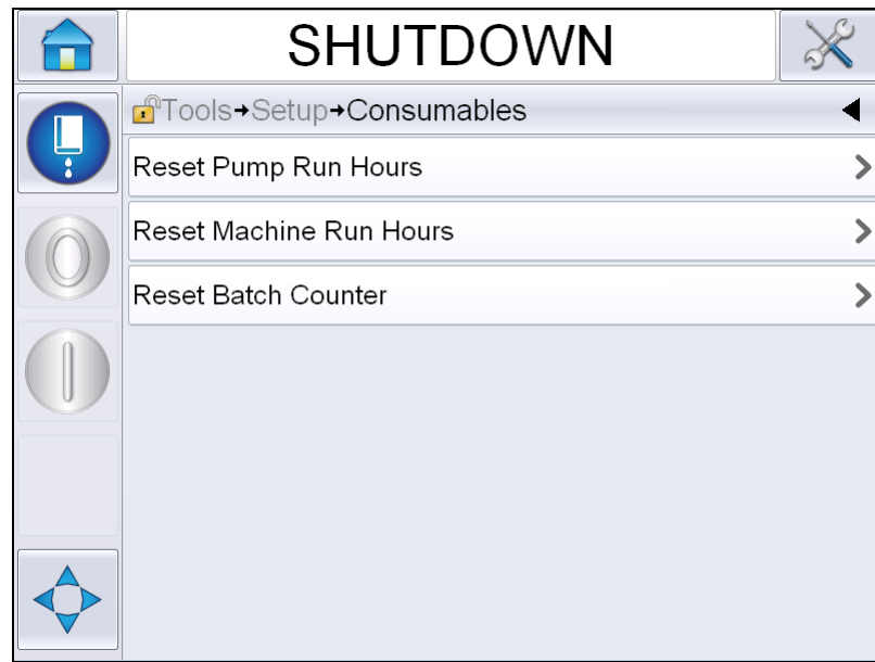
Figure 4-8: Reset Counters
