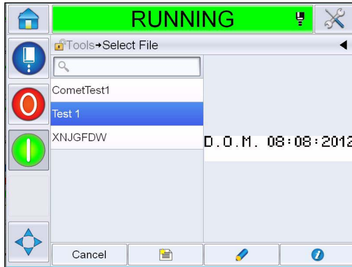
Figure 5-40: Edit Page
