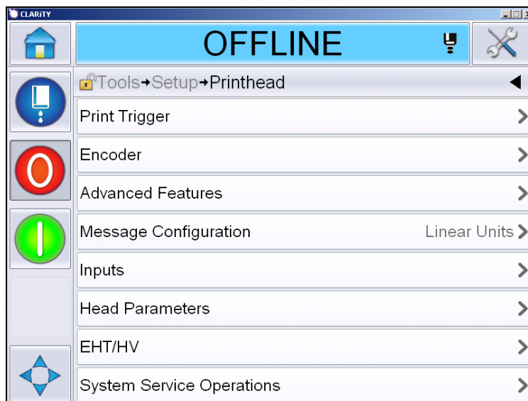
Figure 5-4: Printhead Setting
