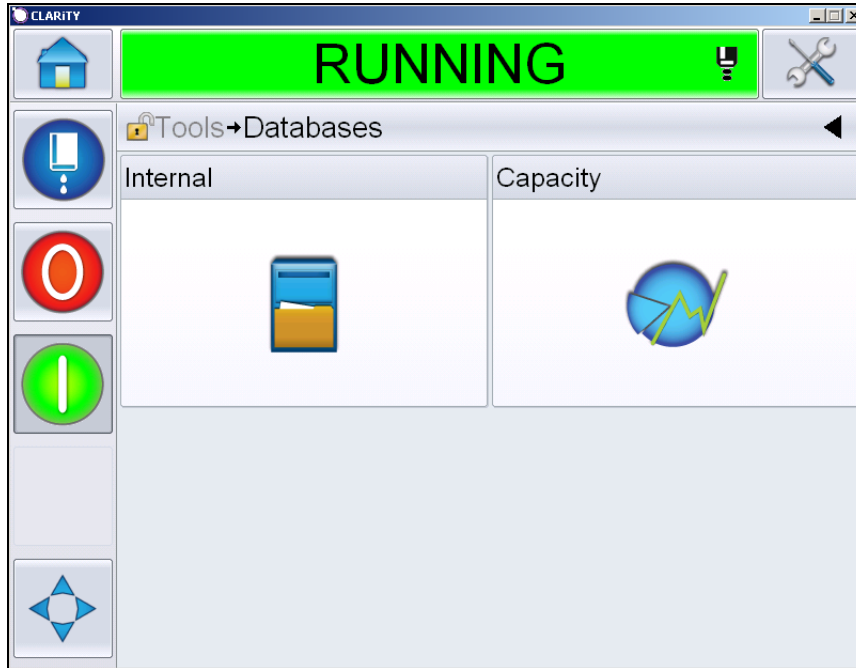
Figure 5-21: Databases
