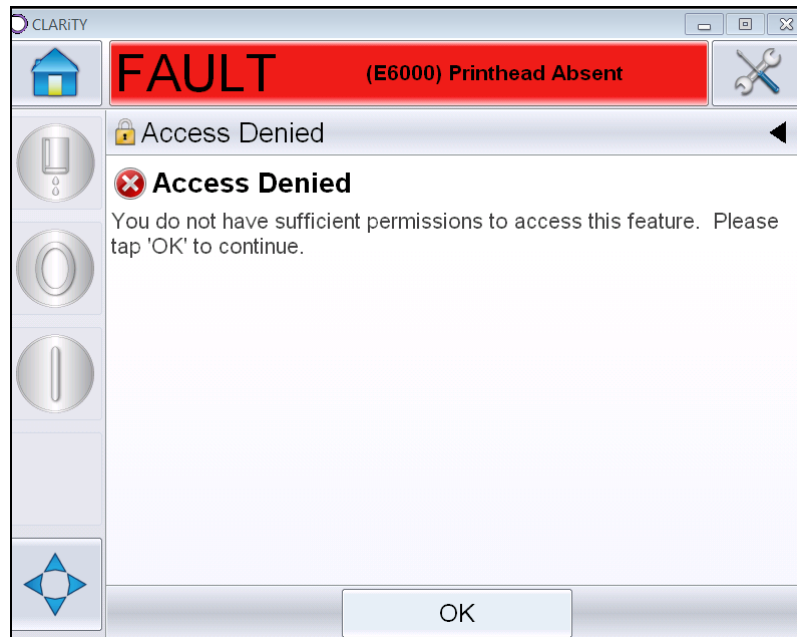
Figure 4-6: Access Denied
