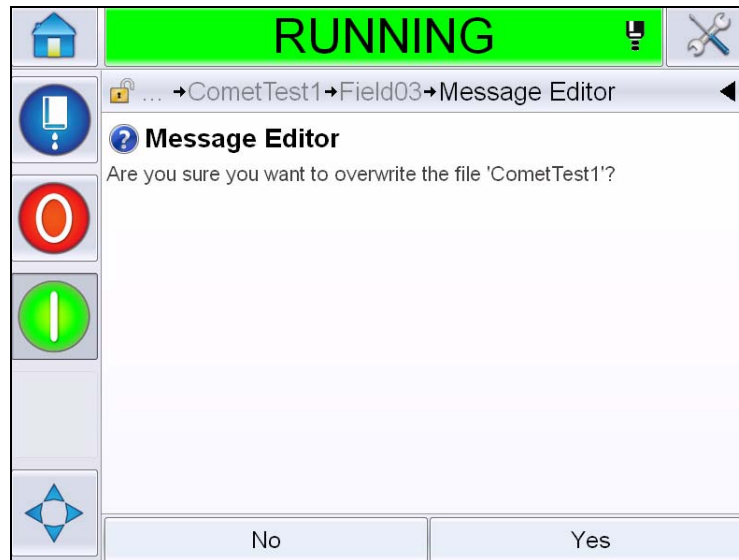
Figure 5-51: Edit Page
