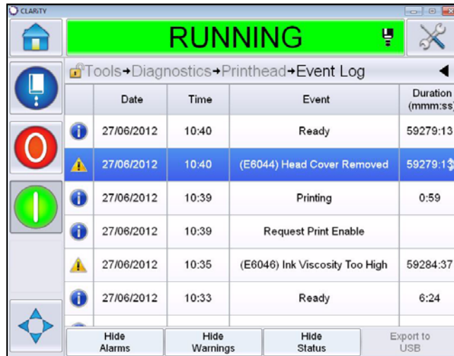
Figure 5-72: Event log
