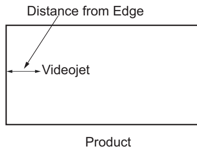
Figure 7-1: Print Position
