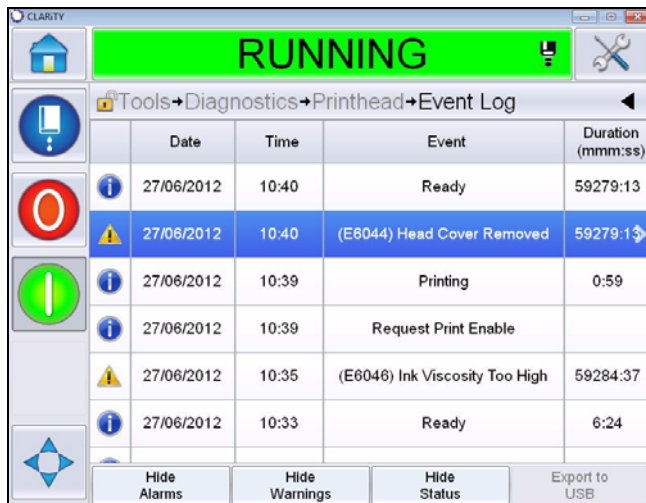
Figure 5-13: Event log
