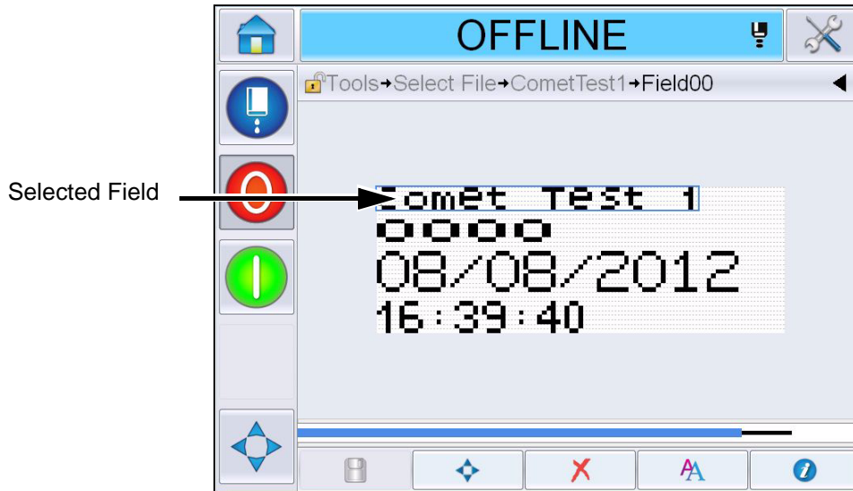
Figure 5-42: Selected Field
