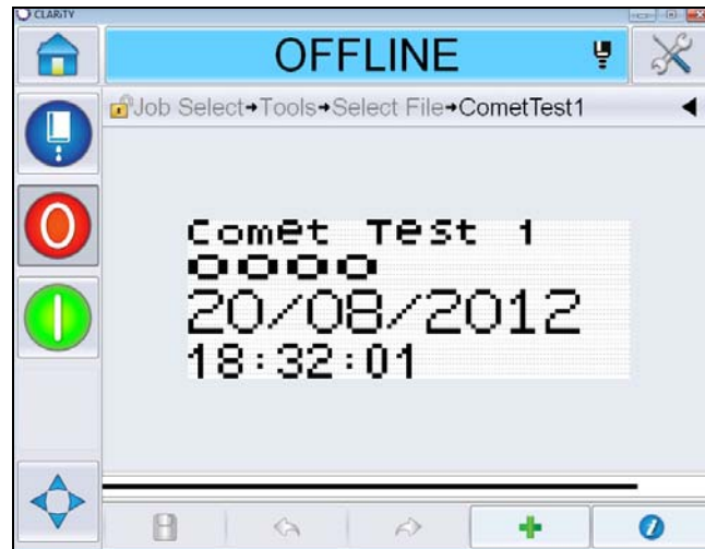
Figure 5-41: Message Page
