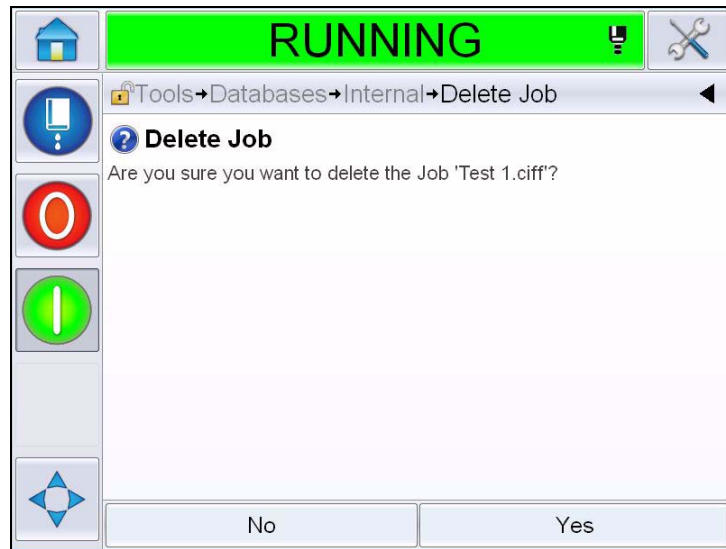
Figure 5-54: Confirmation Screen
