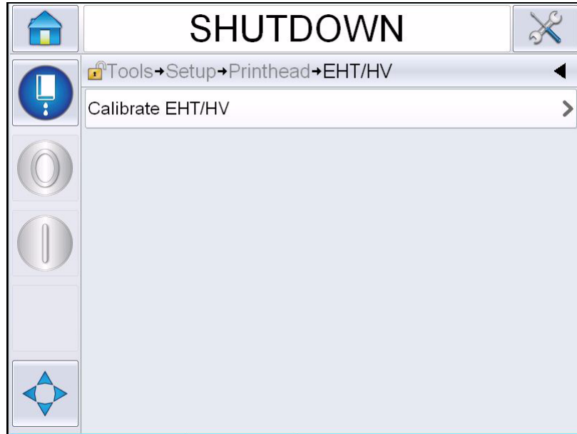
Figure 4-21: EHT/HV Menu
