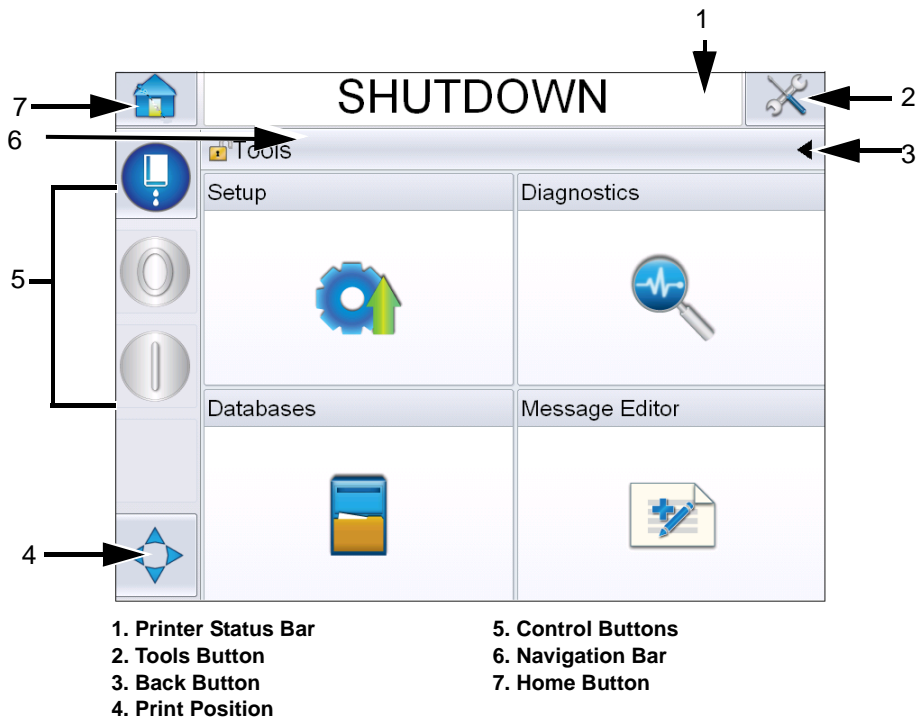
Figure 5-2: Shortcut Icons
